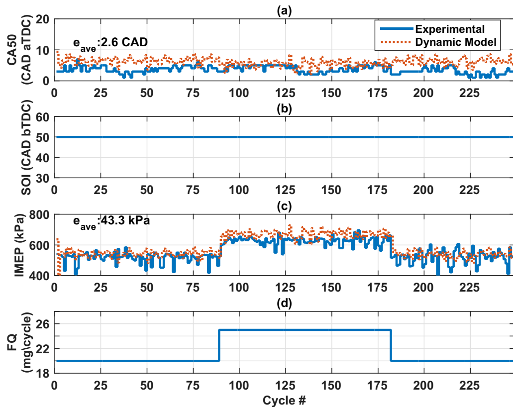
Figure 3.13: Validation of the dynamic model with experimental results for varying FQ, N=1000 RPM, T_{in} = 60^{\circ}C , PR=20 , SOI= 50 CAD bTDC
